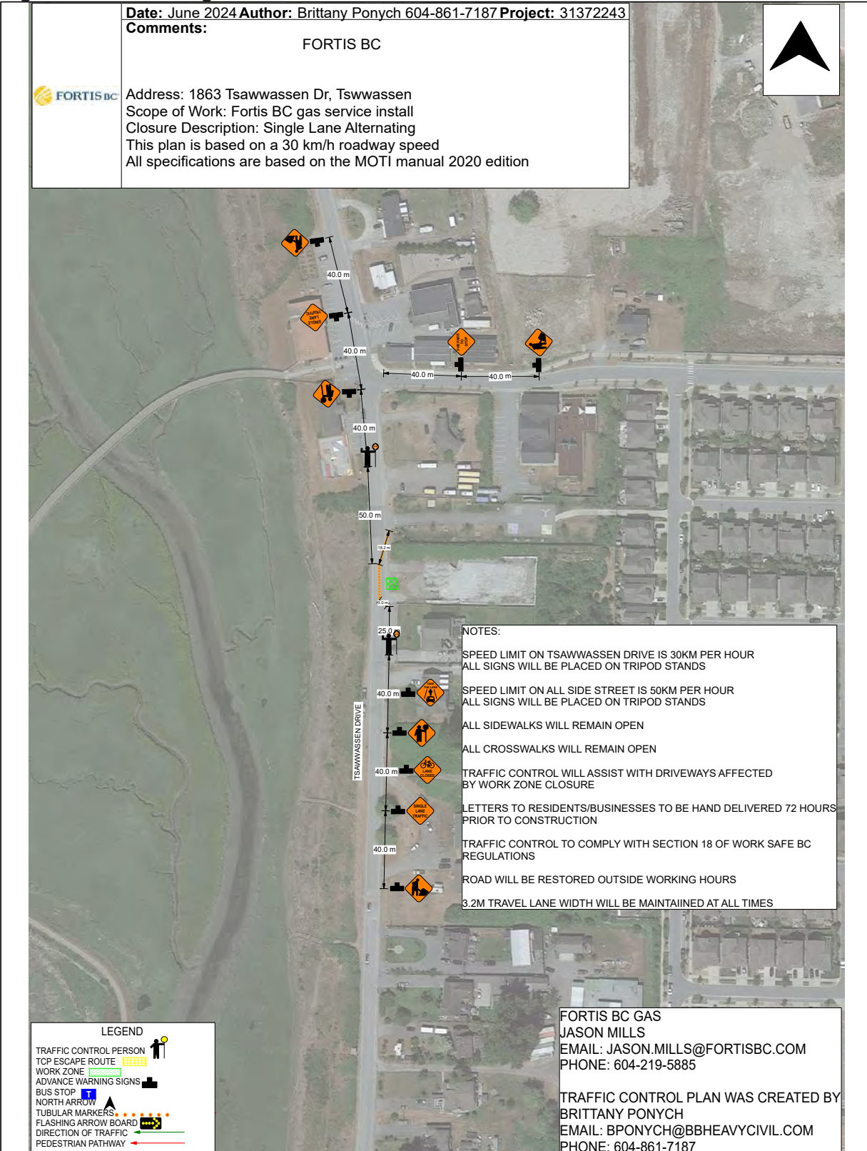
Figure 1: Traffic Management Plan
